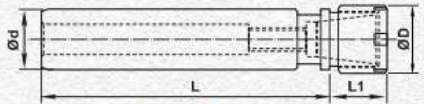
FIG. 1 : With M Type Nut
